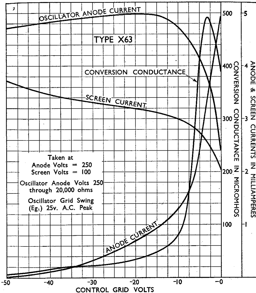
CHARACTERISTIC CURVES OF AVERAGE VALVE.
